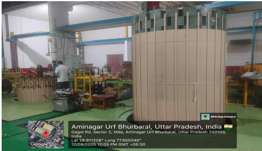
Vapour phase drying oven
