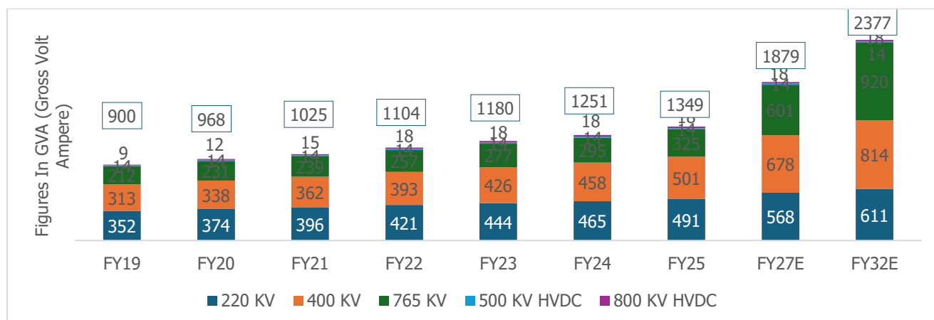
Chart 31: Transformation (Substation) Capacity (220 kV & Above)
