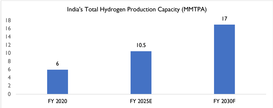
Source: Institute for Energy Economics & Financial Analysis (IEEFA), Press Information Bureau (PIB), D&B Research Estimates *E= Estimated, F= Forecasted
